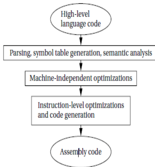
The compilation process
