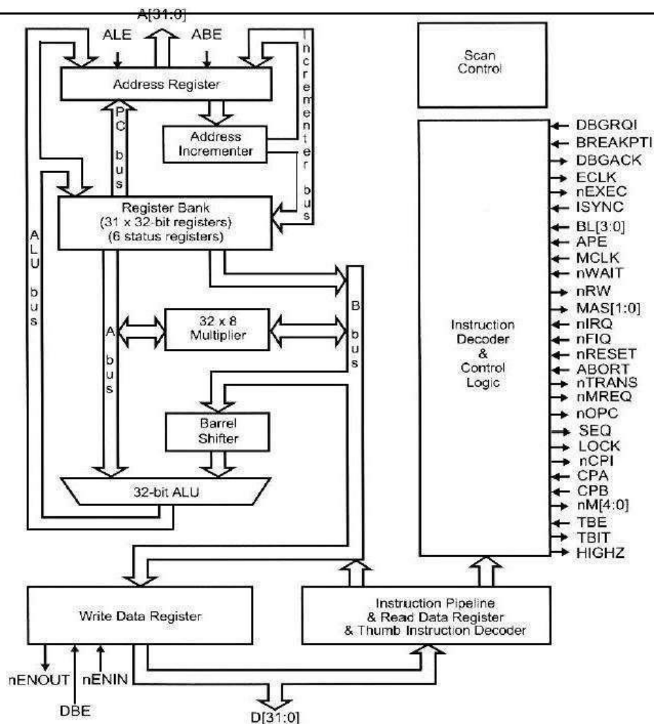
Fig: Architecture of ARM7 Processor.
