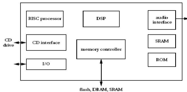
FIGURE 7.22 Architecture of a Cirrus audio processor for CD/MPEG3 players.
